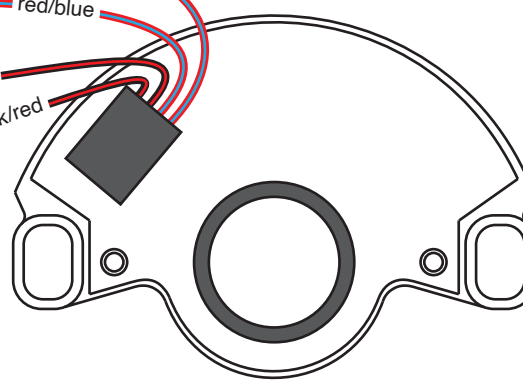
Figure "B" Shown is a typical NSS and Back Up Switch.
