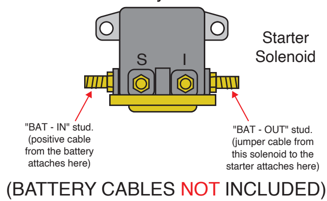
Shown below are the typical "POSITIVE" battery cable connections.
